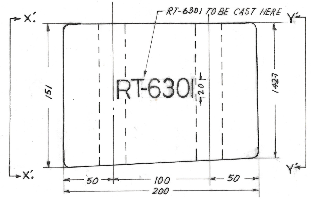
TOP PLAN
